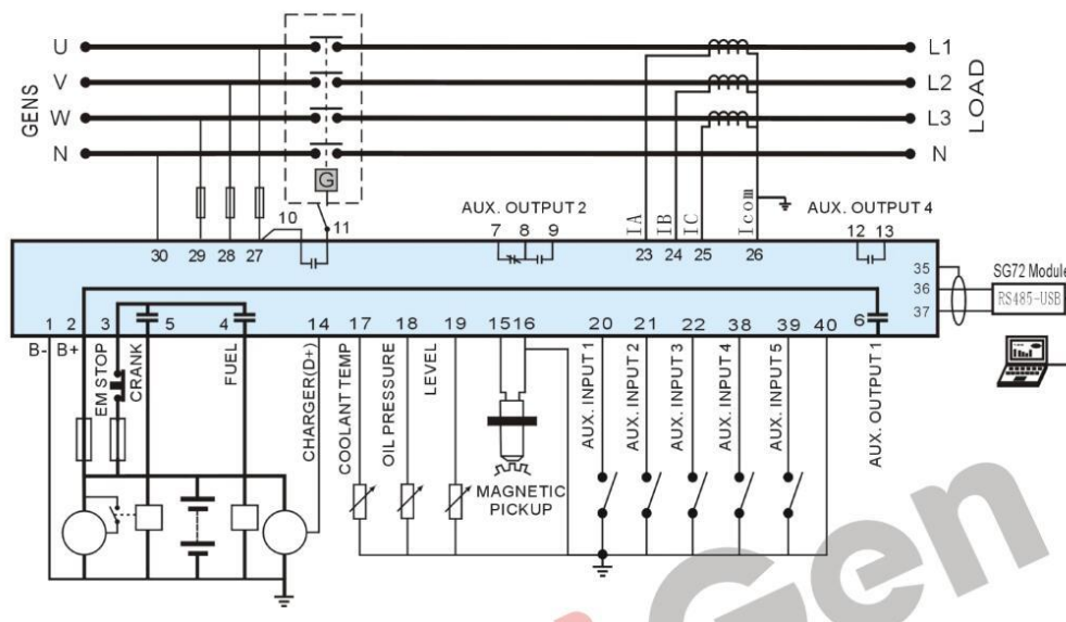
HGM6110NC Typical Application Diagram
